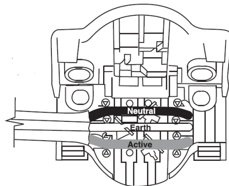
End connection
