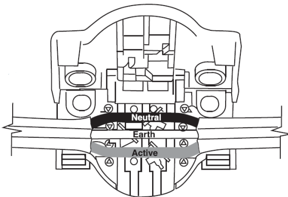
Mid connection
